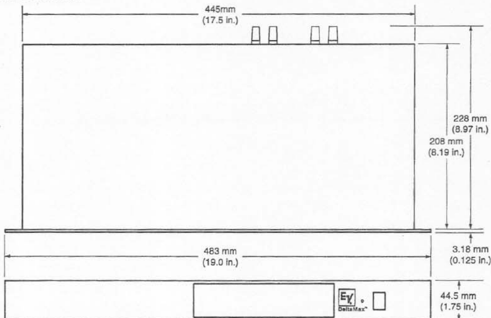
FIGURE 4 — DMC-1122B Dimensions
