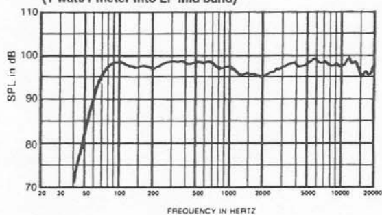
FIGURE 1 — DMC-1122B/DML-1122A Series Frequency Response, on Axis in Anechoic Environment (1 watt/1 meter into LF mid band)
