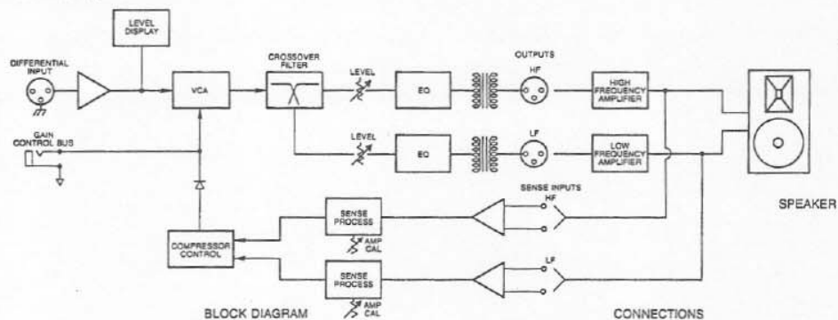
FIGURE 3 — DMC-1122B Block Diagram
