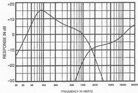
FIGURE 2 — DMC-1122B Frequency Response
